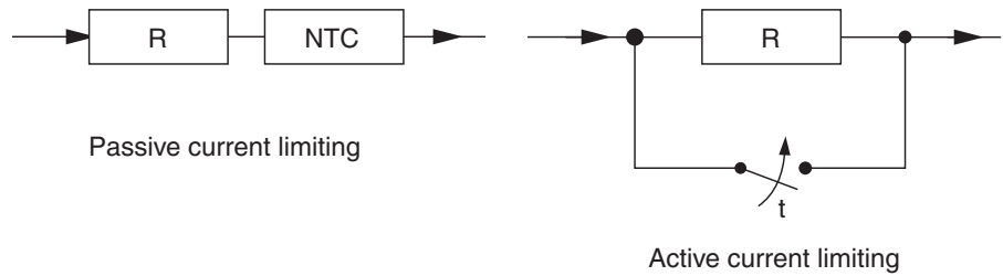
Figure 3-25 Current limiting
